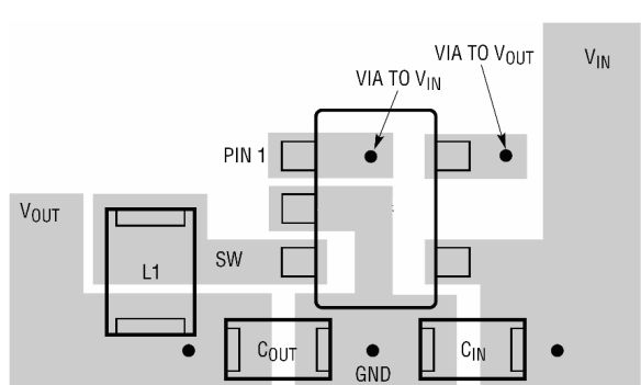
Figure5. APS2410 Fixed output Suggested Layout
