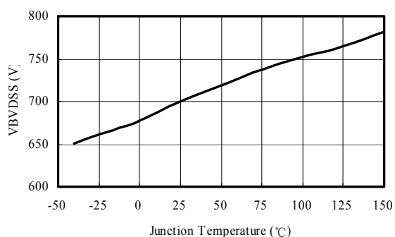
(a) PN6775 BV vs Tj
