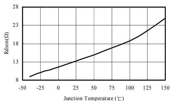
(b) PN6775 Rds(on) vs Tj
